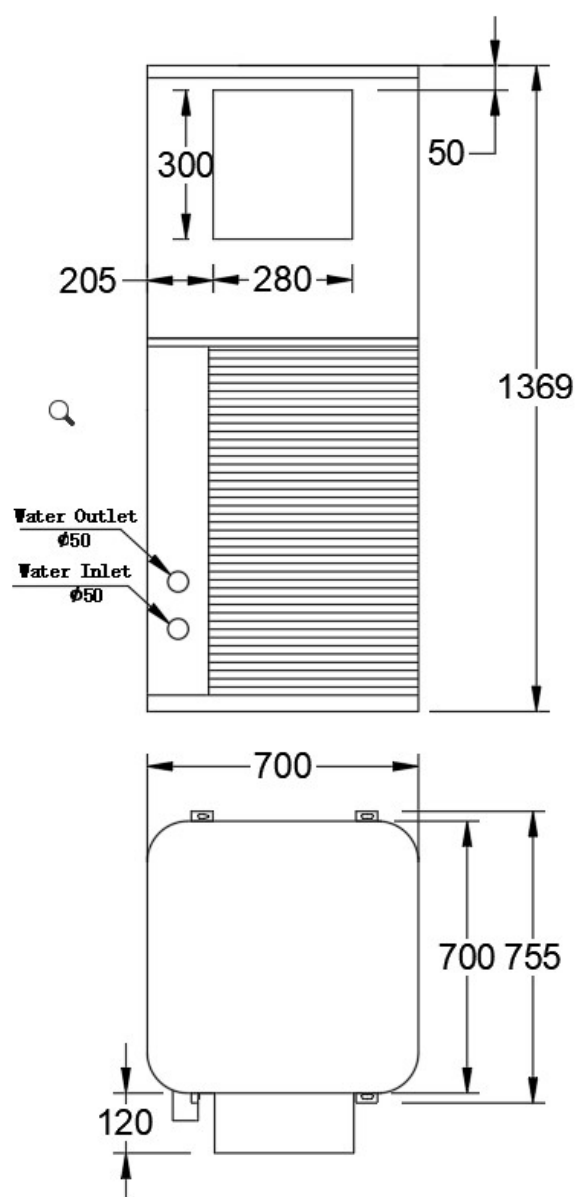
2 – CAHP030S-ZO
