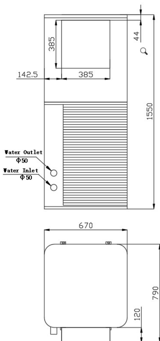
3 – CAHP050S-ZO
