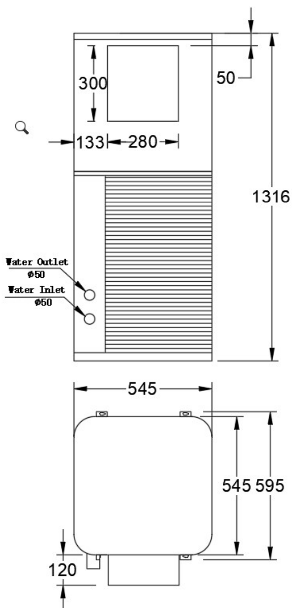
1 – CAHP020S-ZO
