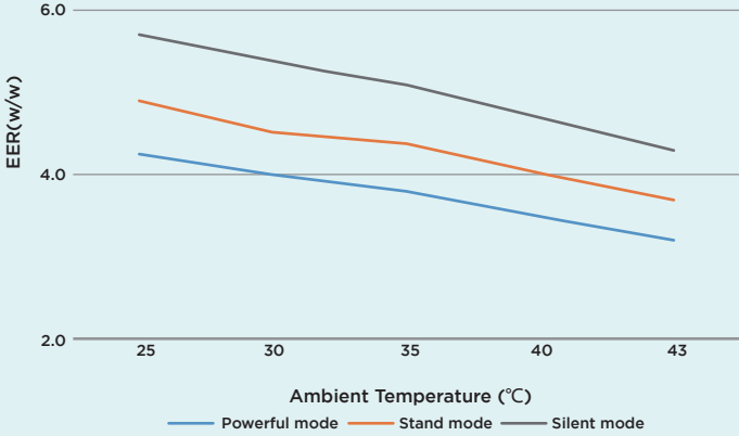
Cooling EER curve
