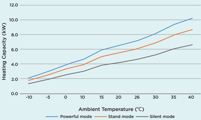
Heating performance curve
