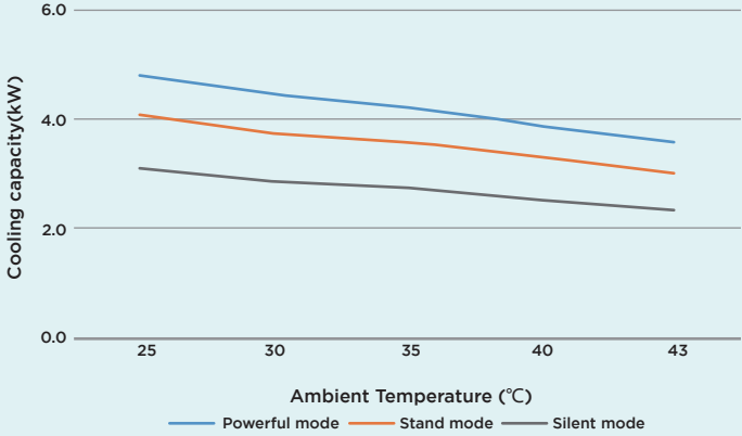
Cooling performance curve
