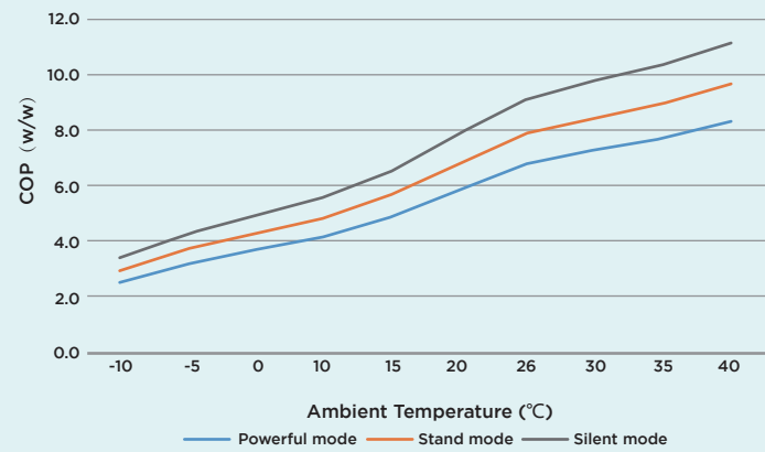
Heating COP curve
